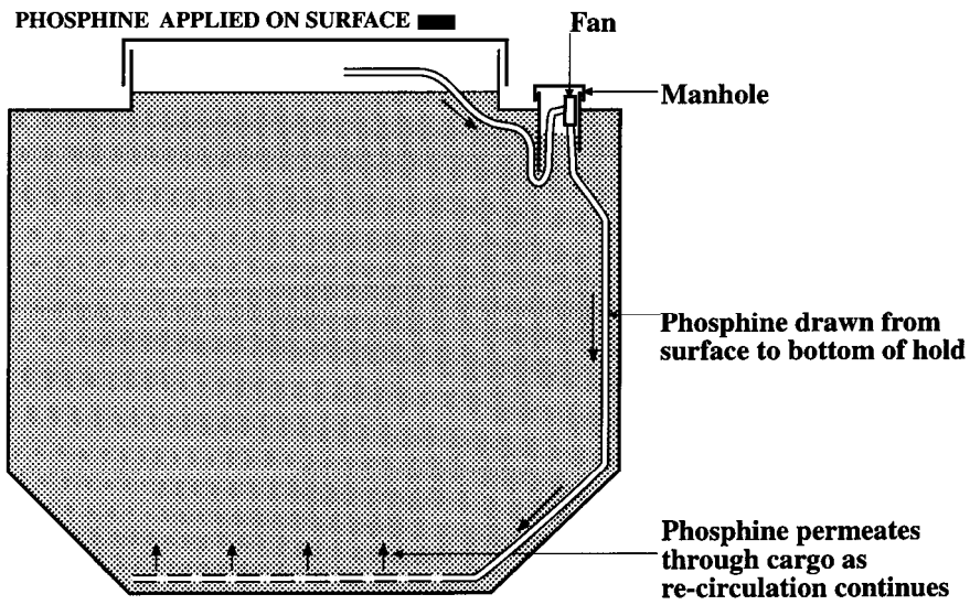
Fig. 2. Fumigation of cargo in ships hold using phosphine and the J. system.
